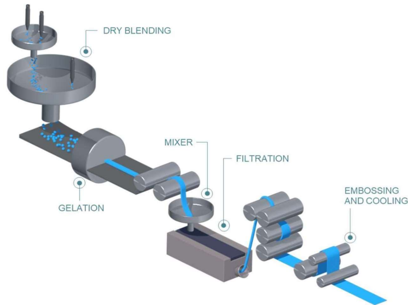
Figure 3: Process flow diagram
